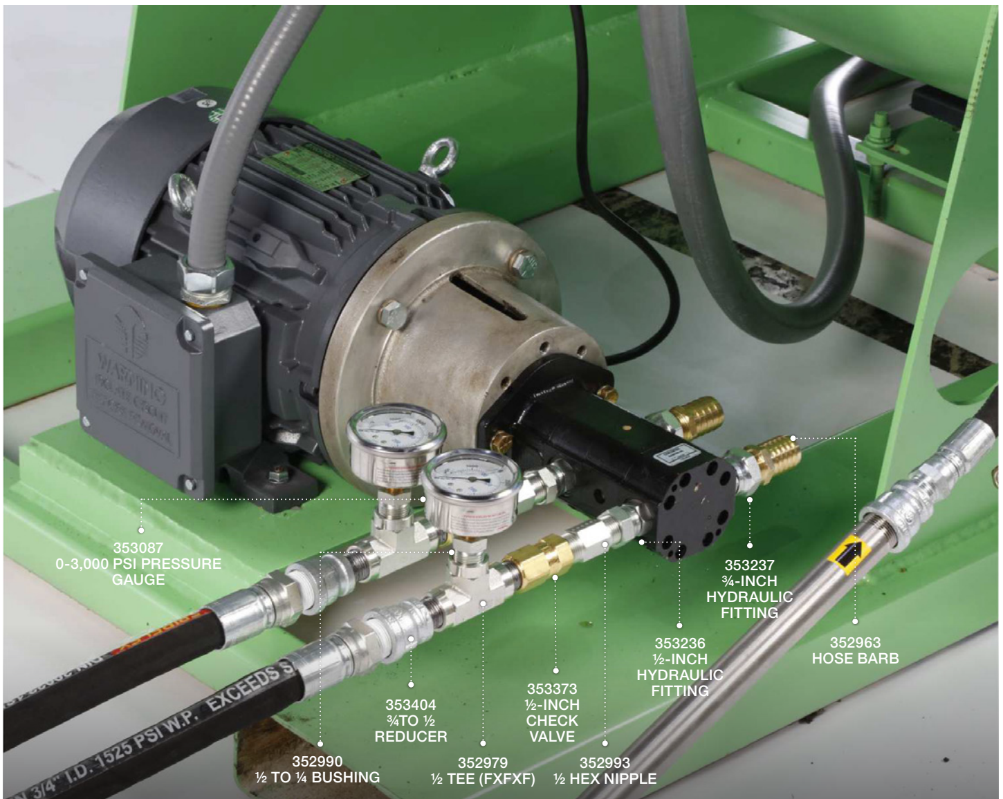
342152 - complete changeover assembly, including all parts shown above as well as the hoses, 3/4-inch manifold (353067), and mixing tube.
